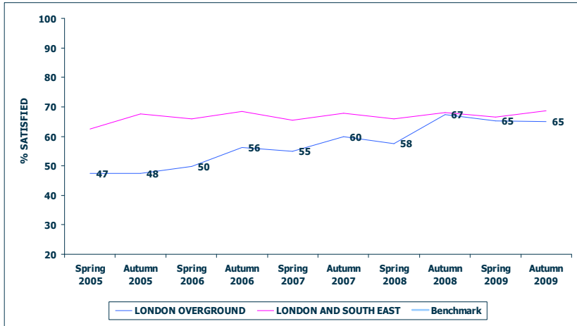
STATION - CLEANLINESS (766)
