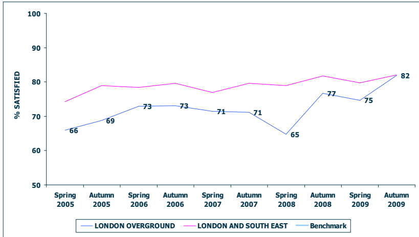
OVERALL SATISFACTION (834)
